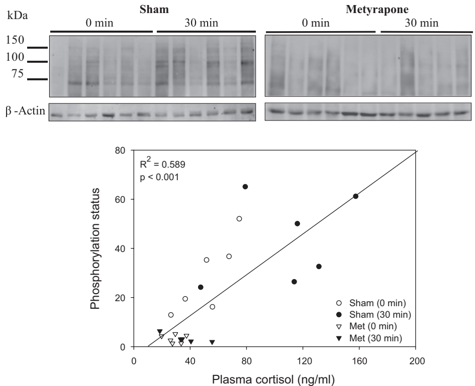
Fig. 5. Effect of acute stress on hepatic protein phosphorylation of protein kinase A (PKA) substrate proteins. Rainbow trout liver homogenates (40 μg of protein) from sham and Met-treated trout before and after acute stress were probed with phospho-PKA substrate polyclonal rabbit antibody (Cell Signaling Technology), which detects proteins that are phosphorylated within the phosphorylation motif for PKA. Protein loading was normalized with β-actin (monoclonal mouse antibody; Sigma). Densitometry values were obtained by quantifying the total phosphorylation intensity of each lane (region shown). The corresponding scatter plot of the plasma cortisol values against the total lane densitometry values is shown. There is a significant positive relationship between plasma cortisol values and PKA substrate phosphorylation ( r^2 = 0.615 , P < 0.001 , n = 23 ).
