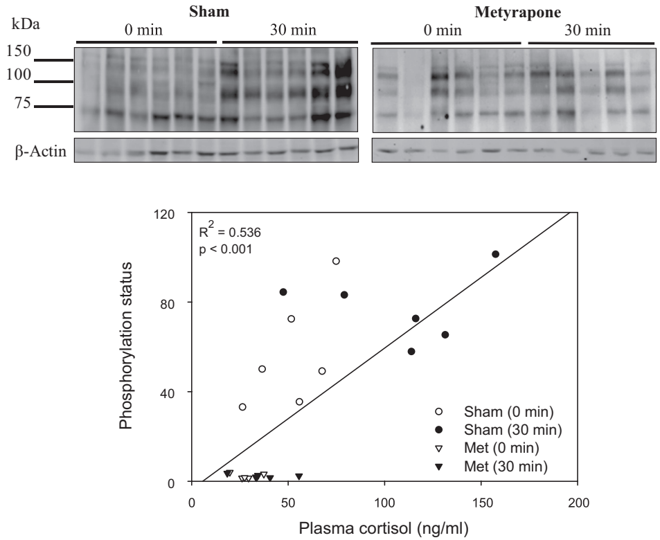
Fig. 4. Effect of acute stress on hepatic protein phosphorylation of protein kinase C (PKC) substrate proteins. Rainbow trout liver homogenates (40 μg of protein) from sham and meyraprone (Met)-treated trout before and after acute stress were probed with phospho (Ser)-PKC substrate polyclonal rabbit antibody (Cell Signaling Technology, Beverly, MA), which detects proteins that are phosphorylated within the phosphorylation motif for PKC. Protein loading was normalized with β-actin (monoclonal mouse antibody; Sigma, St. Louis, MO). Densitometry values were obtained by quantifying the total phosphorylation intensity of each lane (region shown). The corresponding scatter plot of the plasma cortisol values against the total lane densitometry values is shown. There is a significant positive relationship between plasma cortisol values and PKC substrate phosphorylation ( r^2 = 0.607 , P < 0.001 , n = 23 ).
