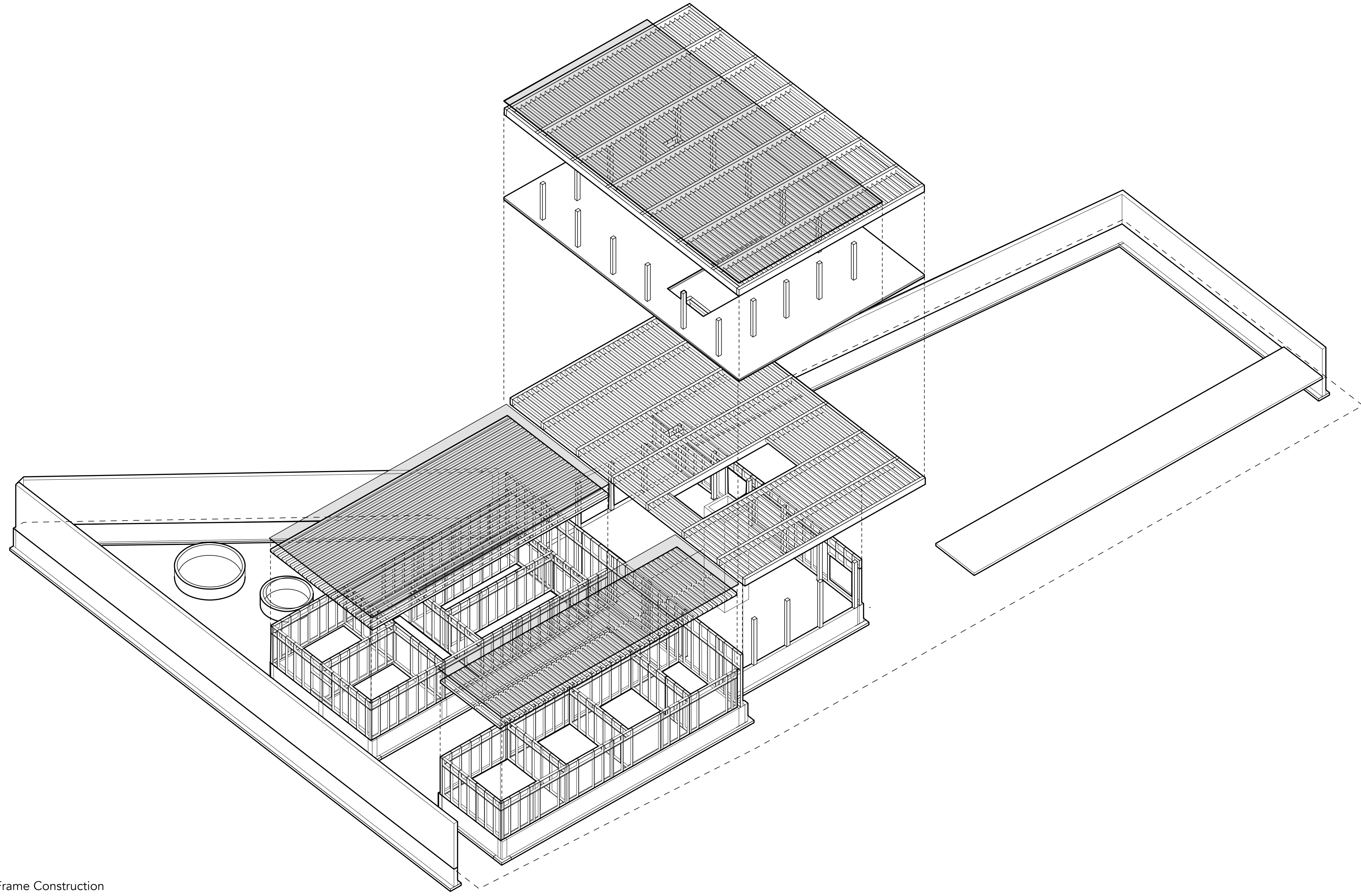
Structural system - Timber Frame Construction
