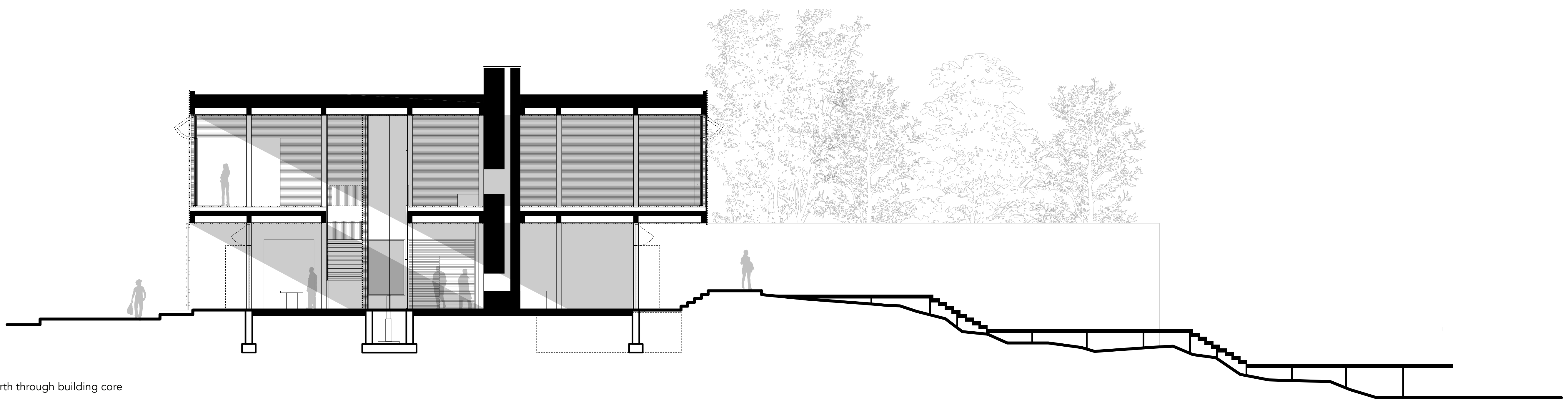
Section 1:100 - Looking North through building core
