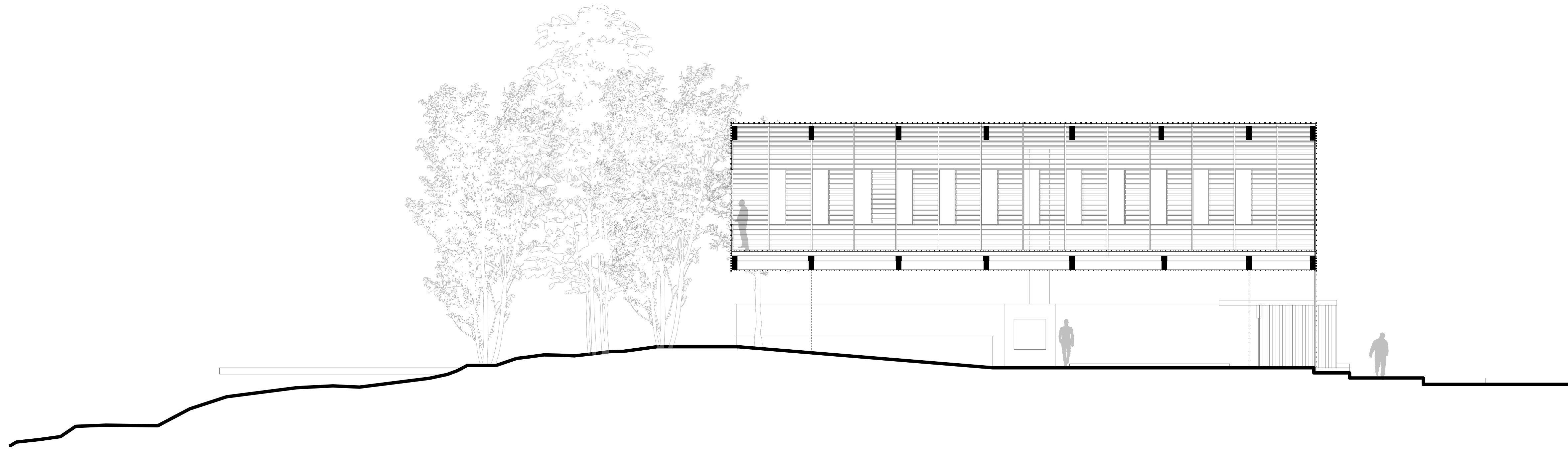
Section 1:100 - Looking South through cantilevered balcony/solarium
