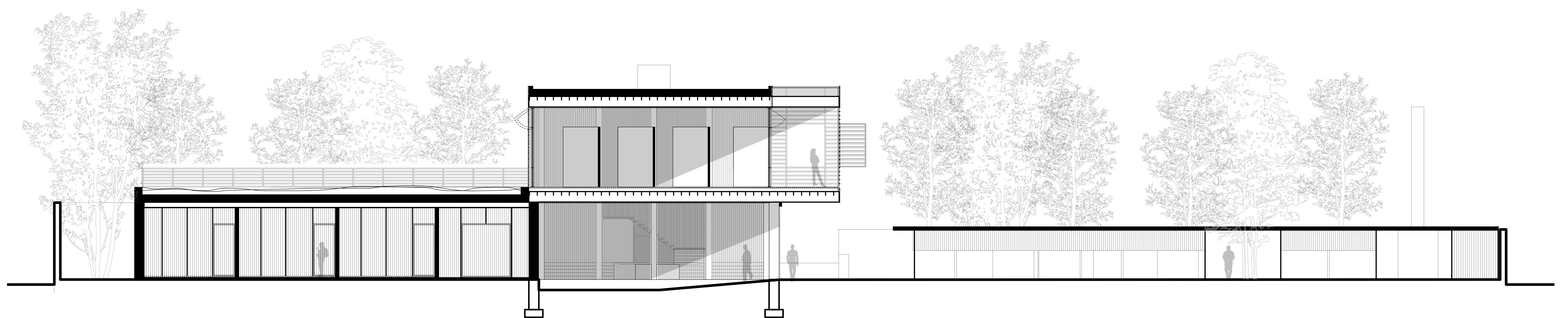
Section 1:100 - Looking East through the practitioner's residences
