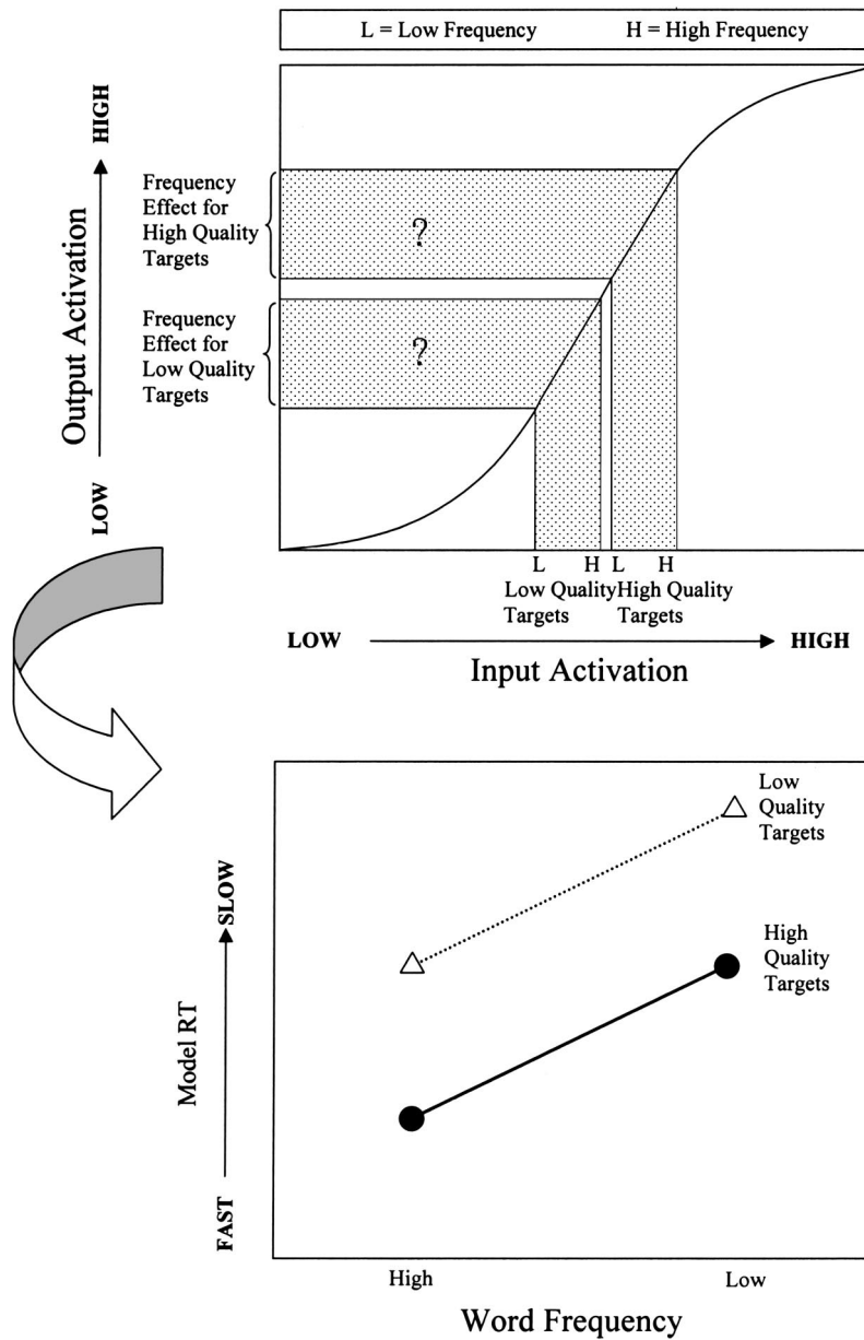
Figure 6. How the sigmoid activation function from the Plaut (1995) and Plaut and Booth (2000) model imposes some problematic constraints when trying to simulate the additive effects of stimulus quality and word frequency. The question marks represent the problematic region of the sigmoid activation function whereby some of the effects that are equidistant from the center of the sigmoid function impose unrealistic constraints on reaction time (RT). A more realistic size of effect of stimulus quality can be modeled by moving closer to the center of the sigmoid activation function (in contrast to Figure 5), but once again, at the cost of no longer accommodating the interactions in Figures 3 and 4.
