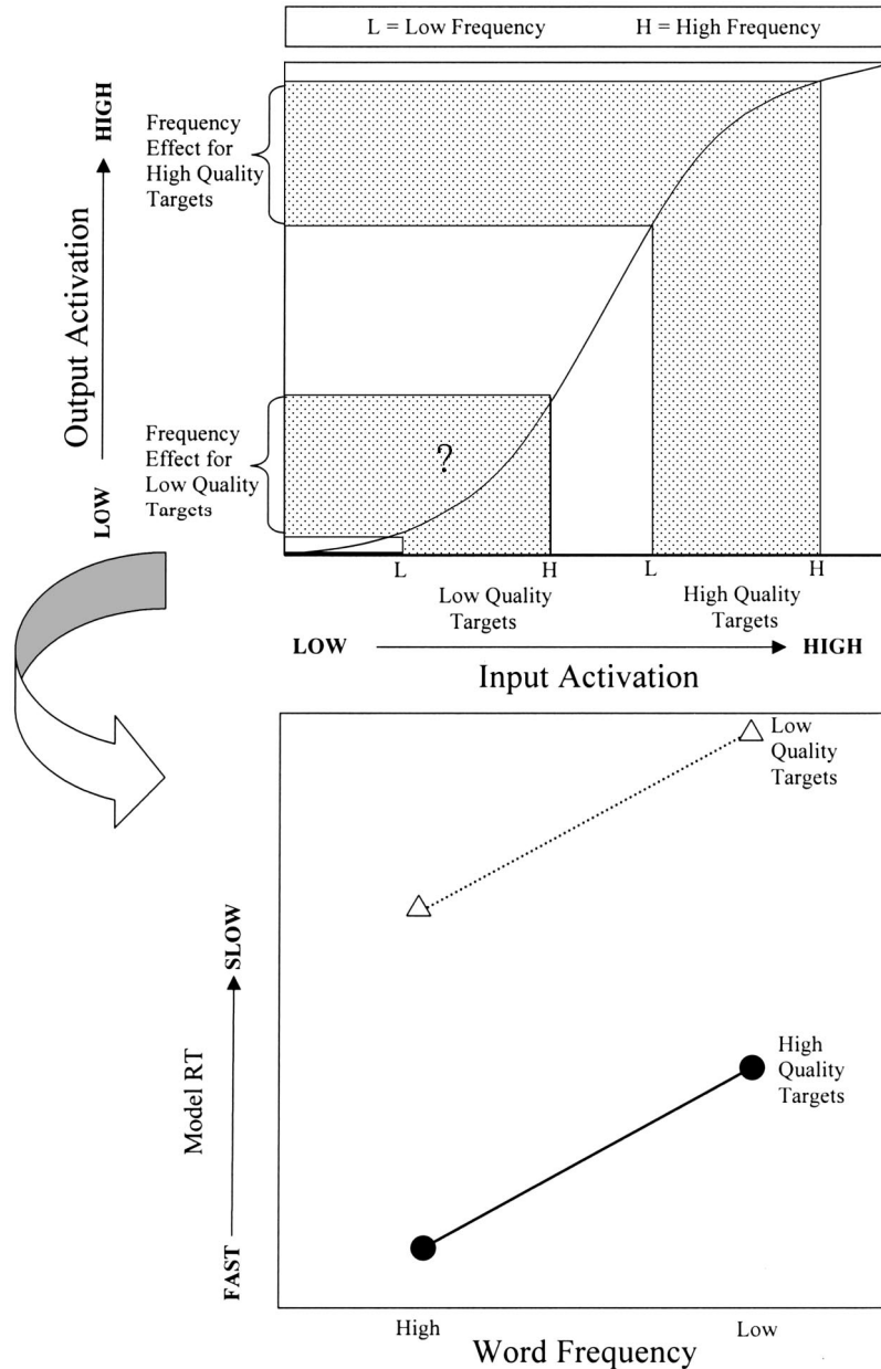
Figure 5. How the sigmoid activation function from the Plaut (1995) and Plaut and Booth (2000) model imposes some problematic constraints when trying to simulate the additive effects of stimulus quality and word frequency. The question mark represents the problematic region of the sigmoid activation function whereby some of the effects that are equidistant from the center of the sigmoid function impose unrealistic constraints on reaction time (RT). If one holds constant the high stimulus quality points from Figures 3 and 4, then the effect of stimulus quality is too large to accommodate the range of RTs of the interaction between context and word frequency (see Figure 4) and the interaction between context and stimulus quality (see Figure 3).
