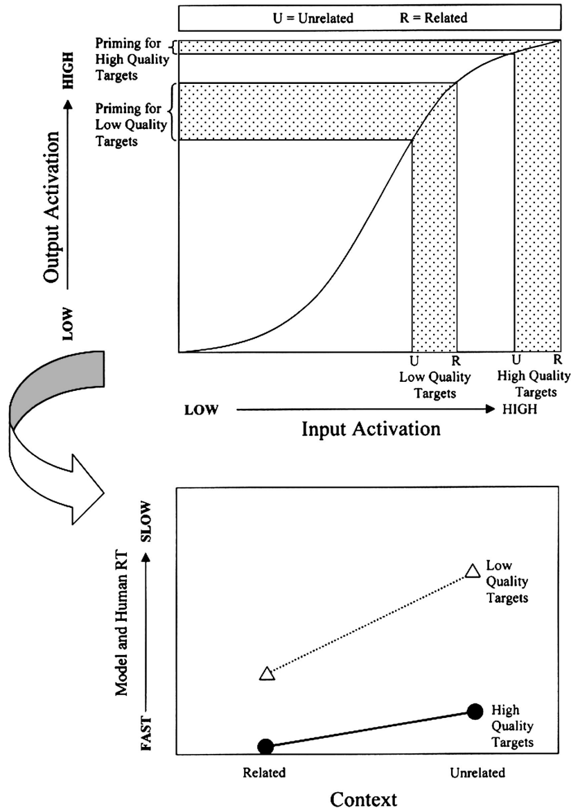
Figure 3. How the sigmoid activation function from the Plaut (1995) and Plaut and Booth (2000) model simulates the interaction between context and stimulus quality. RT = reaction time.
