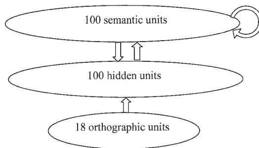
Figure 1. The architecture of the Plaut and Booth (2000) model.
