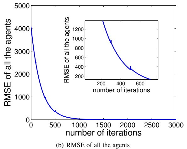
Fig. 5. The effect of results manipulating attack when with our robust algorithm.
