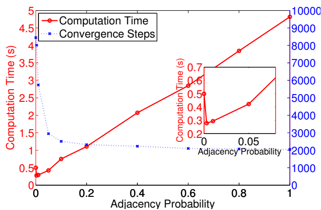
Fig. 3. Total computation time per agent and number of convergence steps versus probability of the ER graph.
