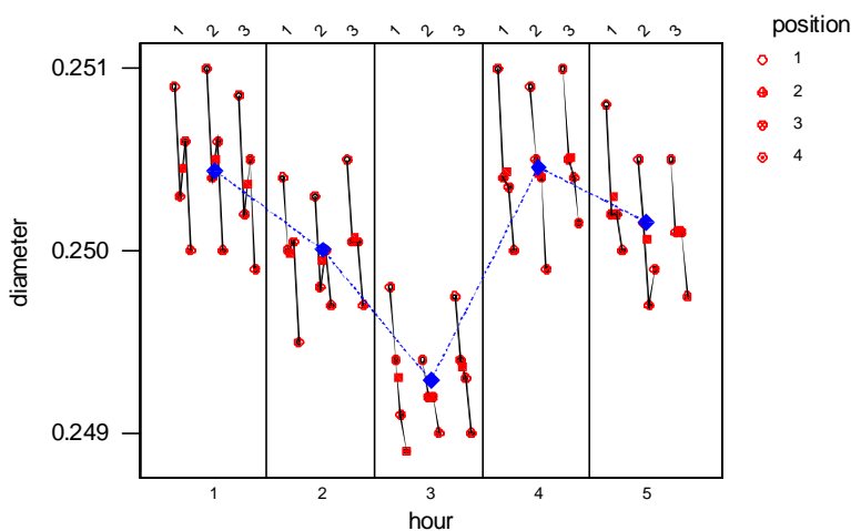
Figure 4: Multivari Chart For Diameter By Position, Piece and Hour
