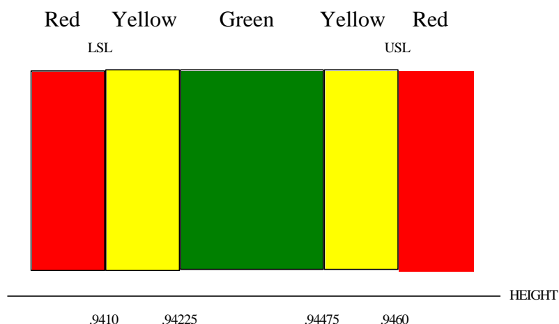
Figure 7: An Example of Precontrol Zones
