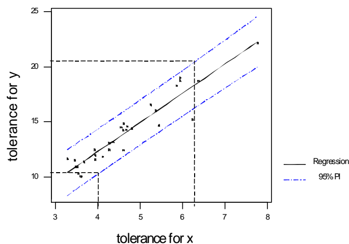
Figure 2: Using Regression to Set Specification Limits (Tolerances) for the Dominant Cause (x) Given a Tolerance for the Output (y)
