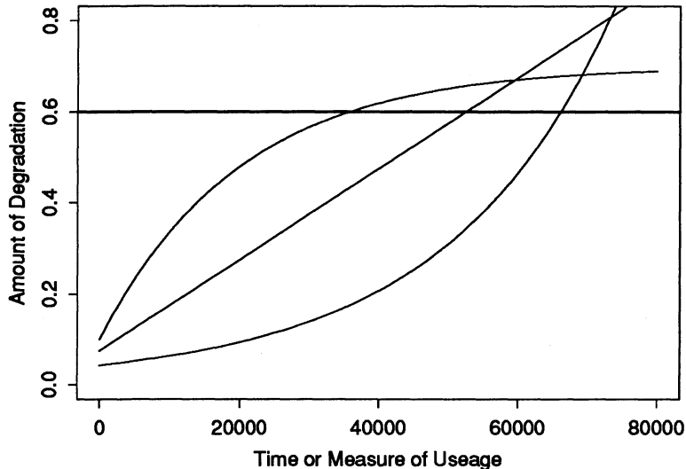
Figure 2: Examples of possible shapes for univariate degradation curves using arbitrary units of degradation and time
