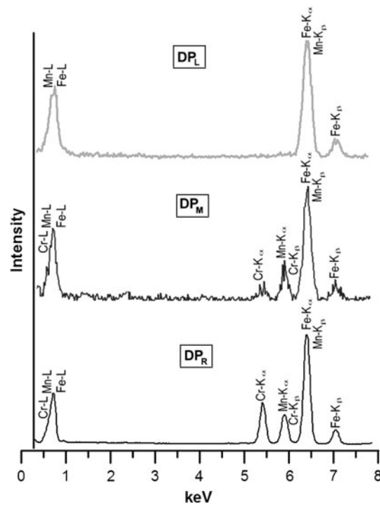
Fig. 7—EDS X-ray spectrums collected from the extracted cementite in nonisothermally tempered DP L , DP M , and DP R specimens.
