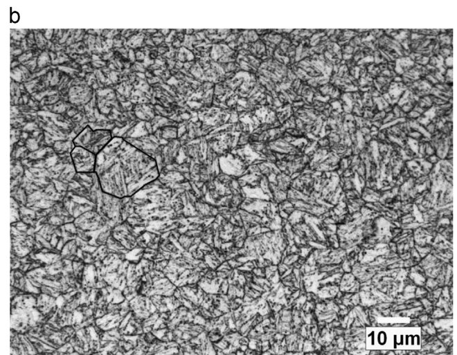
Fig. 5. Optical microstructures of samples tempered at (a) 500 °C for 0.2 s and 600 °C for 10 s. Examples of ferrite grains are outlined.
