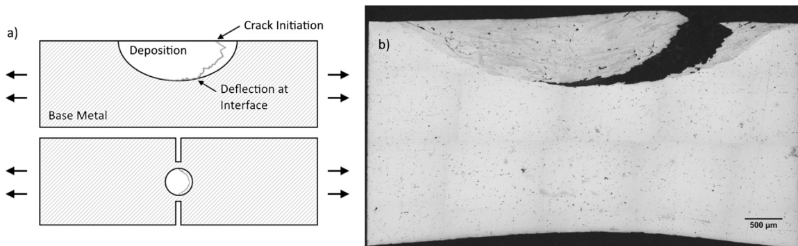
Fig. 7. a) Side and top view schematic of crack location relative to deposition geometry and b) cross-sectional OM image of a lightly etched specimen tested until the initial fracture of the deposited material.
