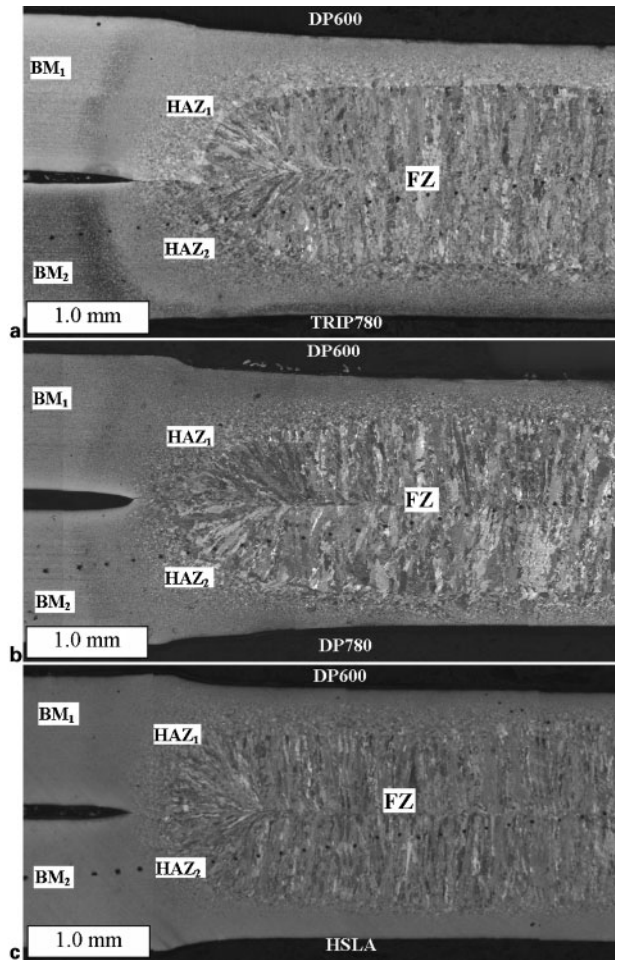
2 Dissimilar spot weld cross-sections: a DP600–TRIP780, b DP600–DP780, c DP600–HSLA FZ – fusion zone, HAZ – heat affected zone and BM – base metal
