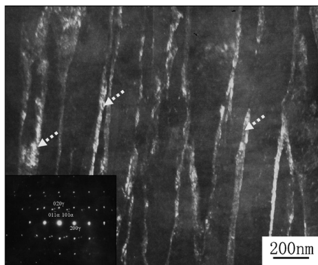
(a) Film-like RA between lathy bainitic ferrite
