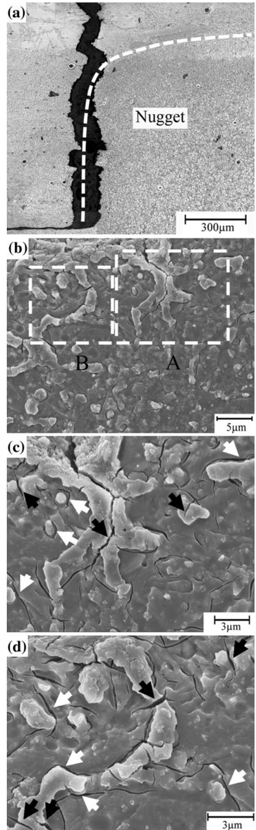
Fig. 7—(a) Typical crack propagation path in the as-welded condition. (b) Microstructure near the crack region for the as-welded sample. (c) Area A at higher magnification. (d) Area B at higher magnification.
