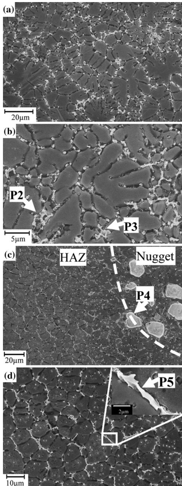
Fig. 3—Typical SEM images of the as-welded microstructure: (a) Microstructure of the fusion zone. (b) High-magnification image from the interdentritic regions. (c) Microstructure of HAZ. (d) Grain boundary particles in HAZ; the EDS analysis results for the highlighted particles are shown in Table I.
