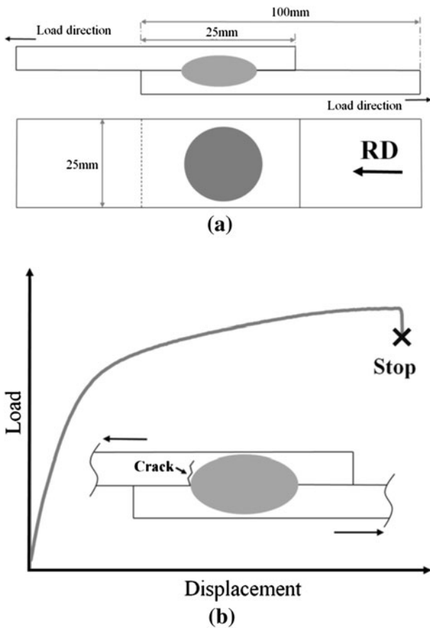
Fig. 1—(a) Scheme of RSW specimens. (b) Scheme of the tensile shear test procedure for assessment of the crack location.
