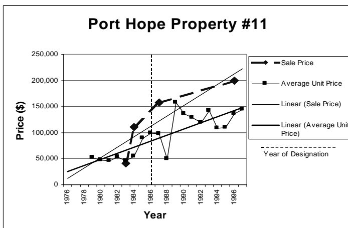
Figure 3 – Regression Analysis
