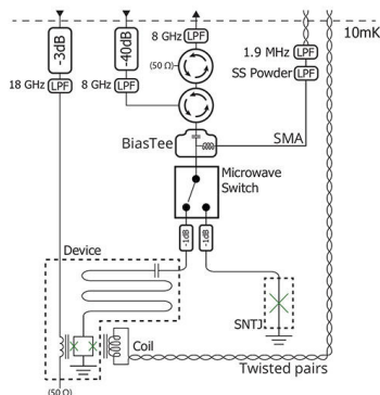
A simplified schematic of the measurement setup.
