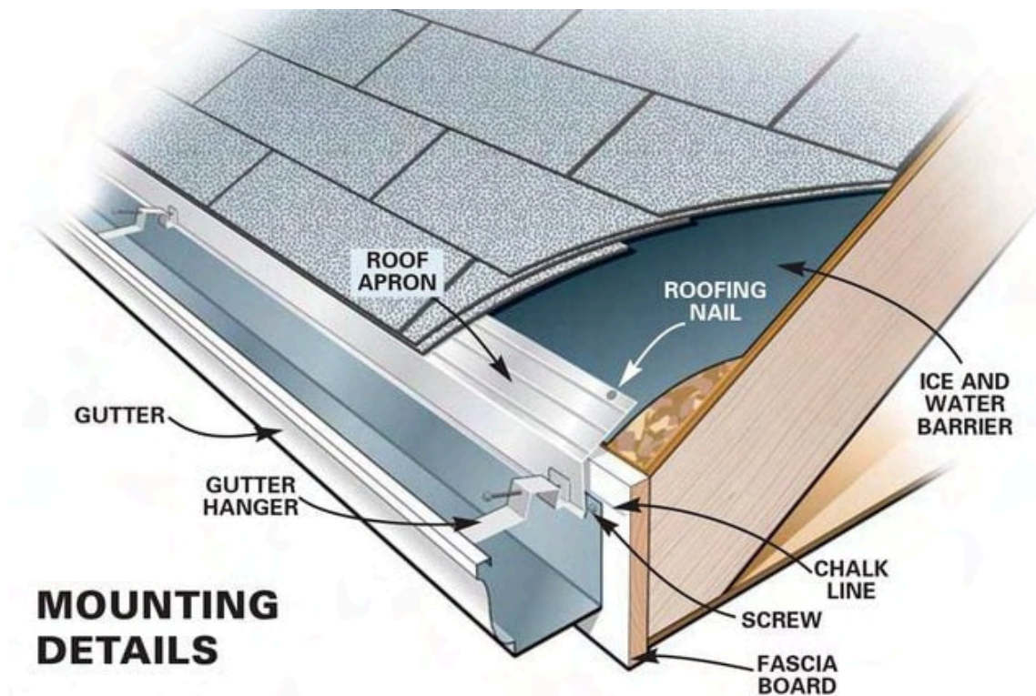
Above: Eavestrough mounting components (Family Handyman, 2024).
