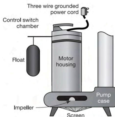
Typical submersible pump
