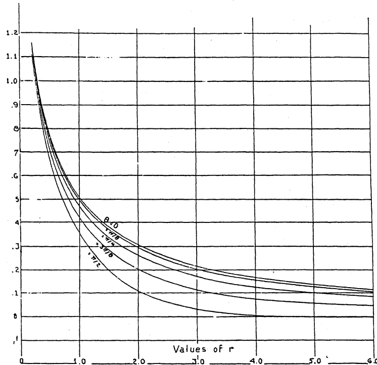
Fig. 3 Q = \text{imaginary part of } J
