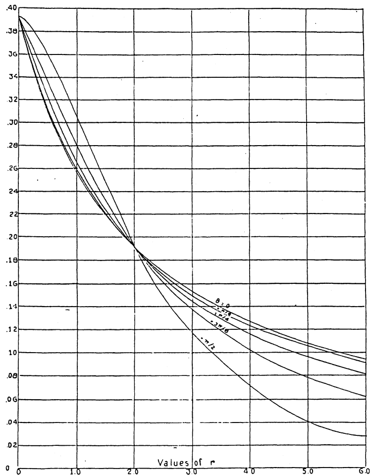
Fig. 2 P = \text{real part of } J
