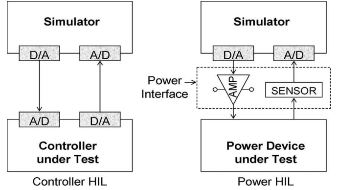
Fig. 3. PHIL and CHIL setup [63].
