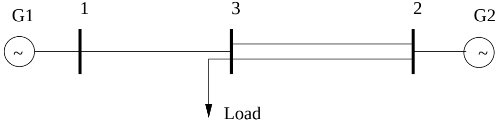
Figure 2.8: IEEE 3-bus test system.
