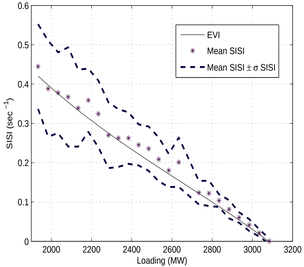
Figure 4.22: SISI for the 2-area benchmark system obtained with use of the subspace method.
