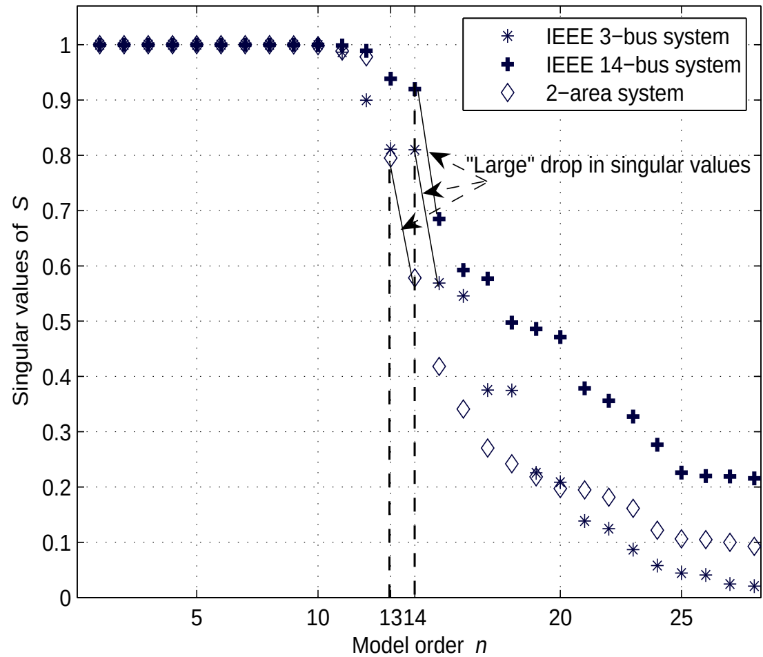
Figure 4.18: Singular values of weighted projection (3.26).
