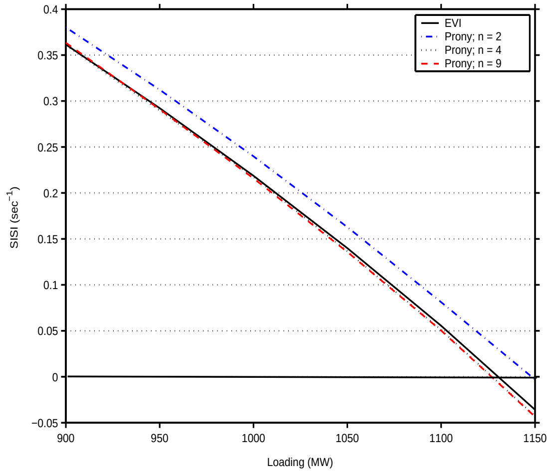
Figure 4.6: Stability index for the IEEE 3-bus system for \text{SNR} = 30 db; line 2-3 outage.
