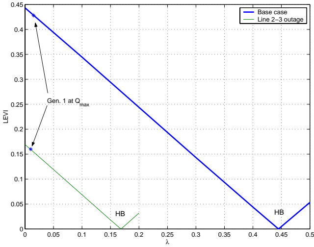
Fig. 6. Linearized eigenvalue index for the three-bus system.
