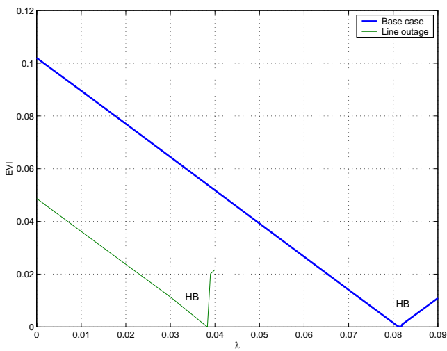
Fig. 10. Eigenvalue index for the two-area system.
