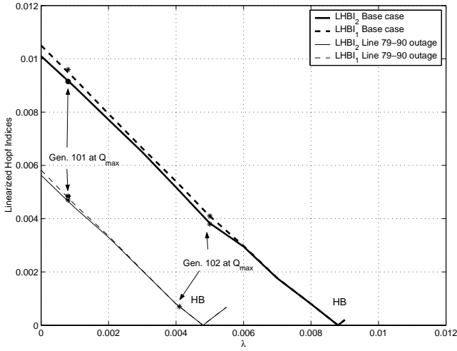
Fig. 19. Linearized Hopf bifurcation indices for the IEEE 50-machine system, Case I.
