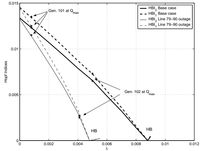
Fig. 17. Hopf bifurcation indices for the IEEE 50-machine system, Case I.
