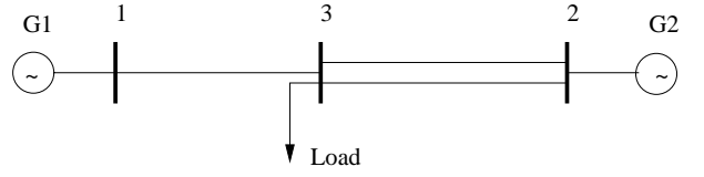
Fig. 1. Three-bus test system.
