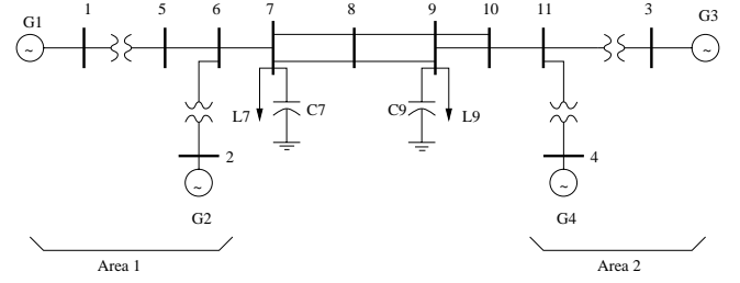
Fig. 8. Two-area test system.
