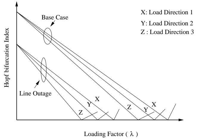
Fig. 28. Hopf bifurcation index for various operating conditions.
