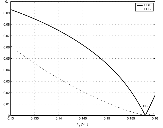
Fig. 27. Hopf bifurcation index and its linearization for the SSR example.
