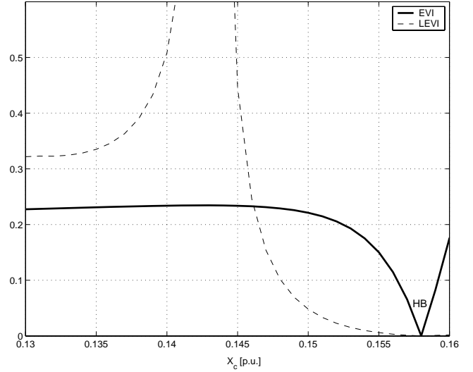
Fig. 26. Eigenvalue index and its linearization for the SSR example.
