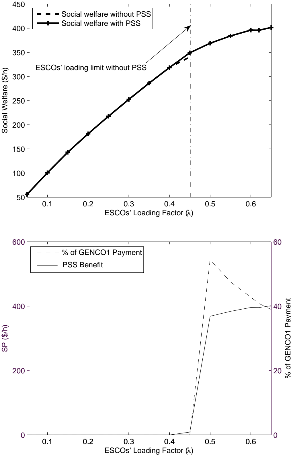
Figure 4.6: S_b and benefits with and without the PSS versus the loading factor for the IEEE 14-bus test system.
