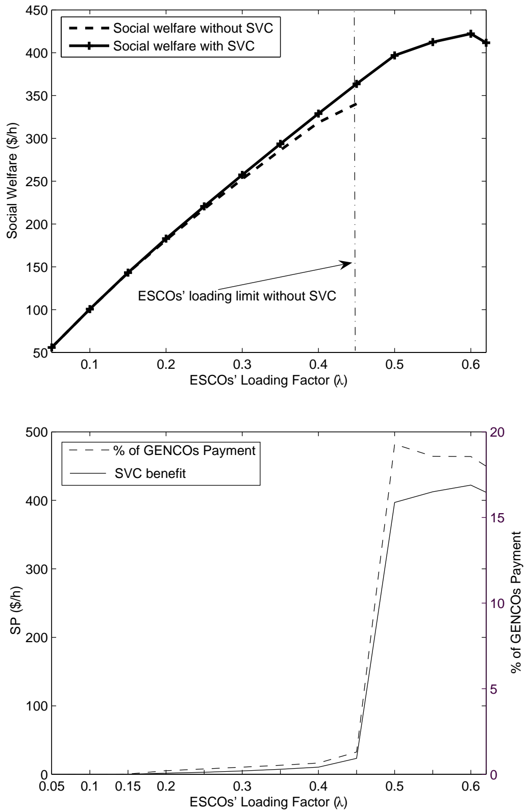
Figure 4.12: S_b and benefits with and without the SVC versus the loading factor for the IEEE 14-bus test system.
