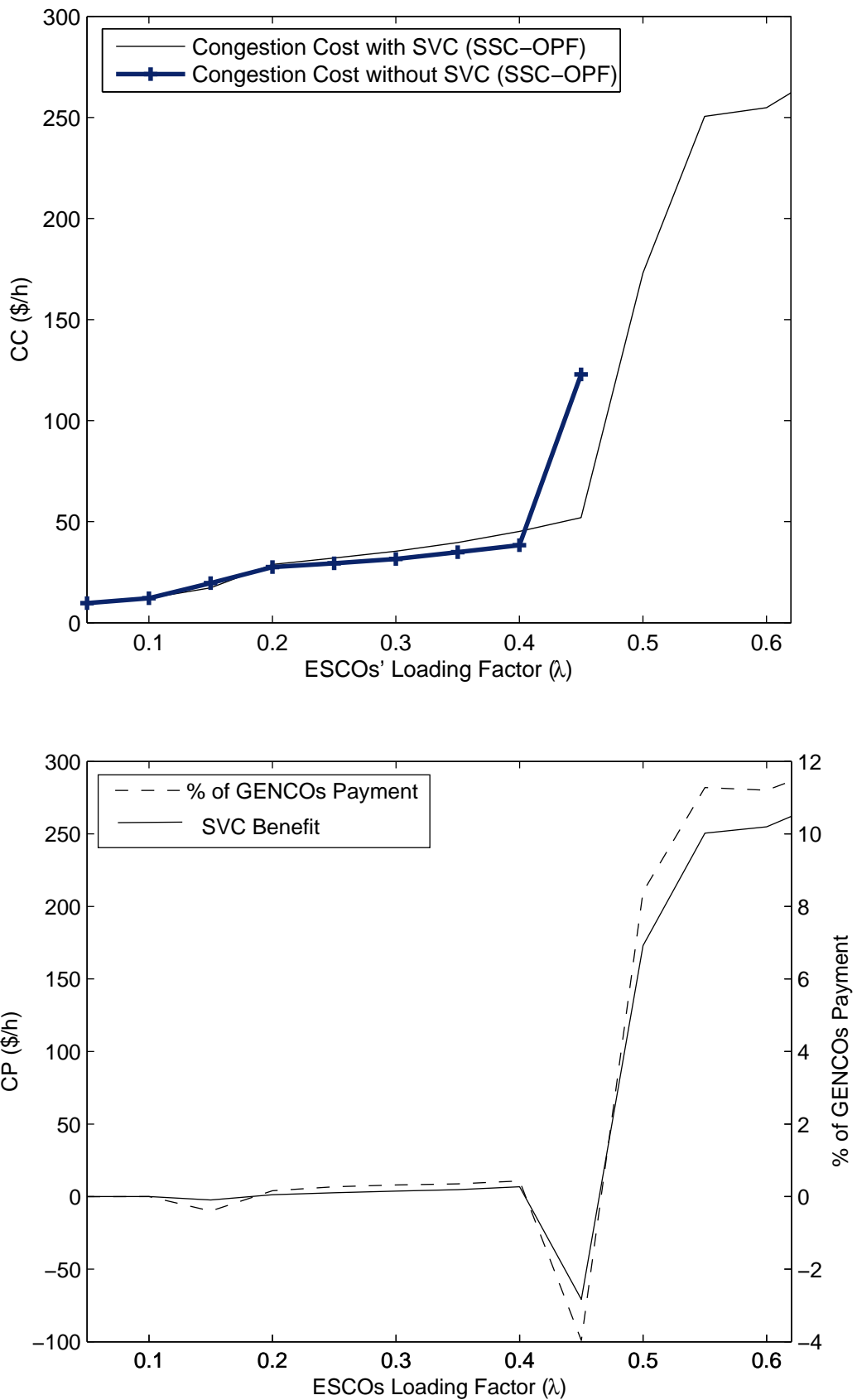
Figure 4.11: SVC benefit and pricing analysis for the IEEE 14-bus test system.
