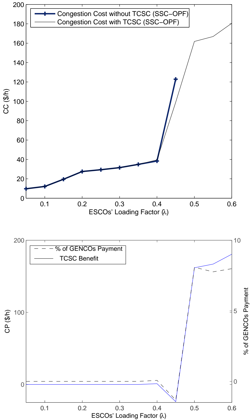
Figure 4.16: TCSC benefit and pricing analysis for the IEEE 14-bus test system.
