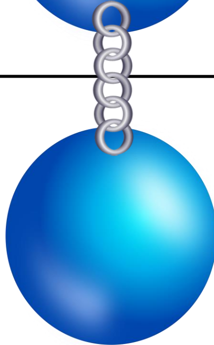
Entangled Qubits
