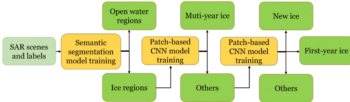
Figure 3. Flowchart of the proposed hierarchical approach for sea ice classification.
