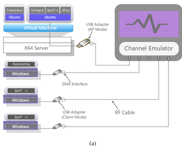
FIGURE 6. Experiment framework. (a) Schematic diagram. (b) Testbed.
