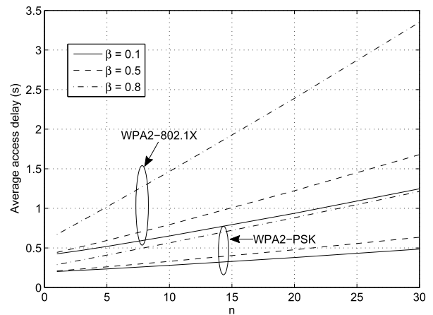
FIGURE 5. Comparison of the access delay performance for the WPA2-802.1X and WPA2-PSK authentication mechanisms.
