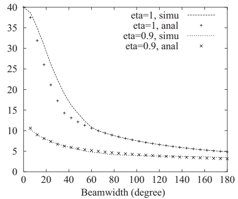
Fig. 6. Number of concurrent transmissions, case 4.
