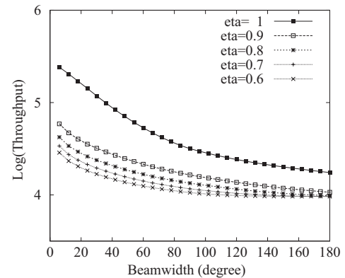
Fig. 7. Throughput with different antenna efficiency, case 4.
