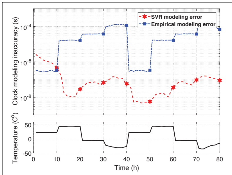
FIGURE 4. The modeling accuracy with the help of the SVM algorithm is significantly enhanced compared to the empirical model used in traditional clock synchronization methods. With fluctuating and inhospitable operating environments, sub-microsecond modeling errors are always attainable by utilizing the proposed SVM-based scheme.
