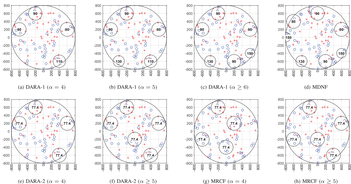
Fig. 6. DSC placement scenarios (Case Study I).
