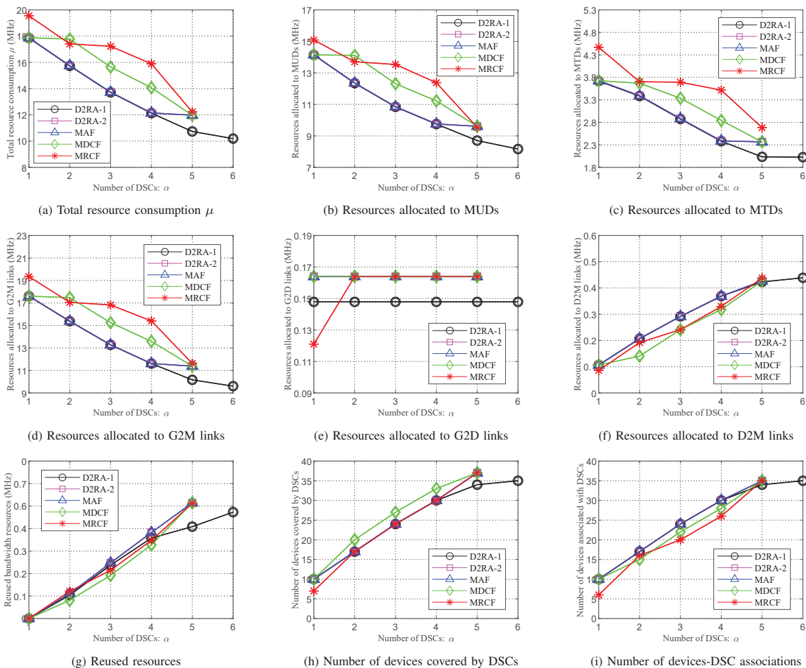
Fig. 5. Impact of the number of available DSCs (Case Study I).
