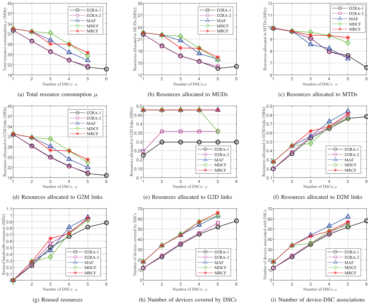
Fig. 7. Impact of the number of available DSCs (Case Study II).
