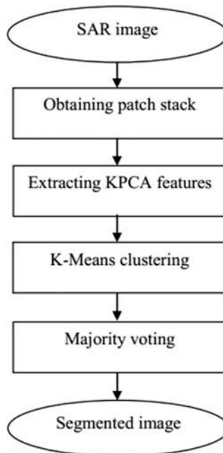
Figure 5. The flowchart of the proposed segmentation scheme.
