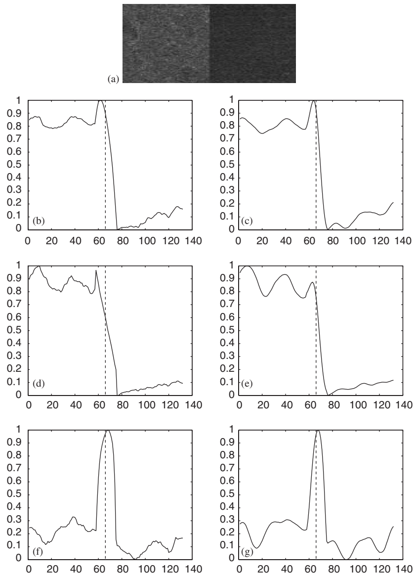
Fig. 3. Edge transects for SAR ice-water bi-partite image for selected feature statistics. Original test image included. (a) SAR ice-water image, (b) GLCP: entropy results, (c) WGLCP: entropy results, (d) GLCP: contrast results, (e) WGLCP: contrast results, (f) GLCP: correlation results and (g) WGLCP: correlation results.
