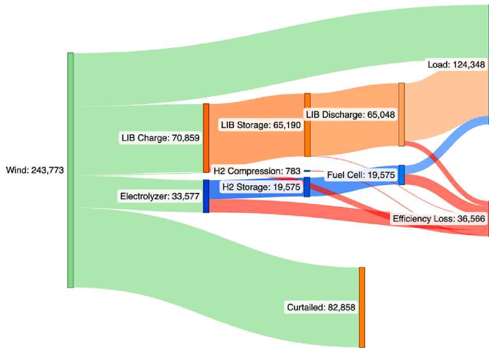
Fig. 4. Annual Energy Flows, 2020 Hybrid Base Case. Unit is MWh. Total generation is 196% of the load. 49% of all generation is either curtailed (34%) or lost due to conversion/storage efficiency (15%). Load is met roughly equally by the wind electricity directly (55%) and energy storage (45%). The LIB subsystem accounts for 88% of the load met by energy storage and receives 68% of the wind electricity directed to energy storage.
