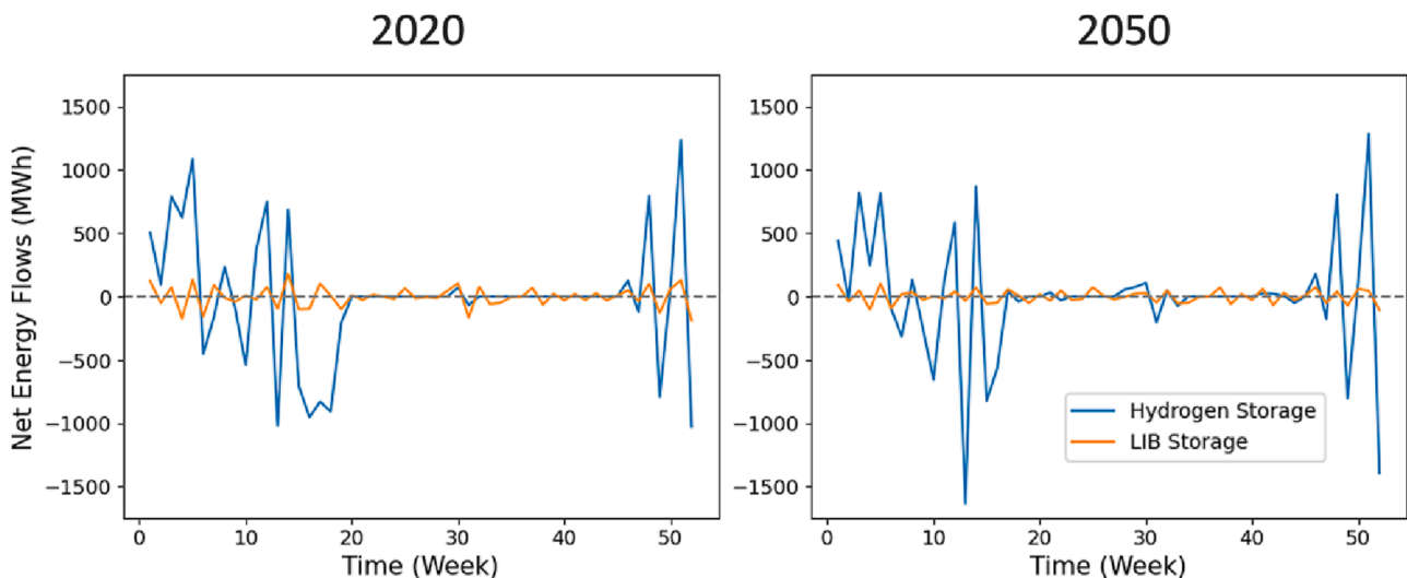
Fig. 3. Weekly Net Energy for the H 2 and LIB Subsystems. Net energy is calculated as the sum of energy entering into storage (after efficiency losses) minus energy leaving storage (before efficiency losses). Values above zero indicate that H 2 or LIB is supplying energy to the system.
