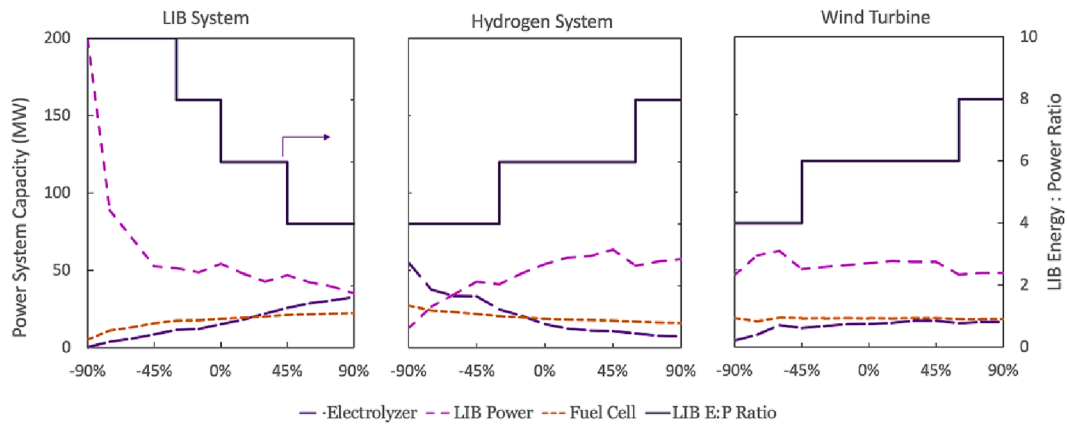
Fig. 9. Impact of Subsystem Costs on Component Sizing and the LIB Energy-Power. The left, middle, and right graphs show the impact of LIB subsystem, H 2 subsystem, and wind turbine cost on system composition, respectively. To change subsystem cost, the annualized cost of each component of the subsystem was changed by the same percentage. Dashed lines are the power conversion components, and the solid line is the LIB energy-power ratio.
