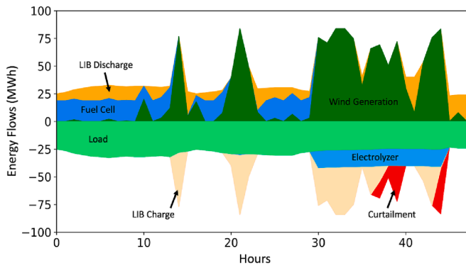
Fig. 2. Hourly Energy Flows Through All Components of the Microgrid (First 48 Hours of the 2020 Hybrid Base Case). Positive values correspond to energy supply, and negative values correspond to energy consumption.
