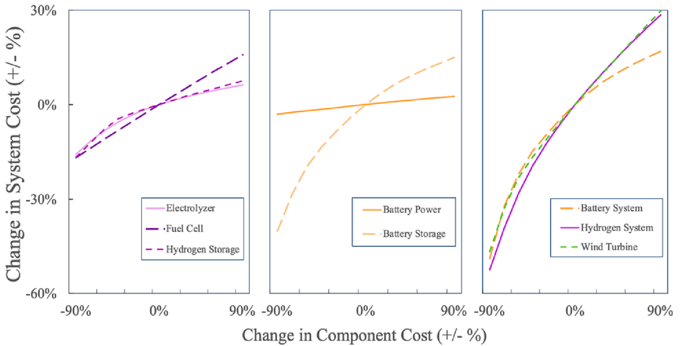
Fig. 7. Impact of the Cost of Different Technologies and Subsystems on Total Microgrid Cost. Components of the H 2 subsystem (left); Components of the LIB subsystem (middle); energy storage and wind farm subsystems (right). To change subsystem cost, the annualized cost of each technology in the subsystem was changed by the same percentage.
