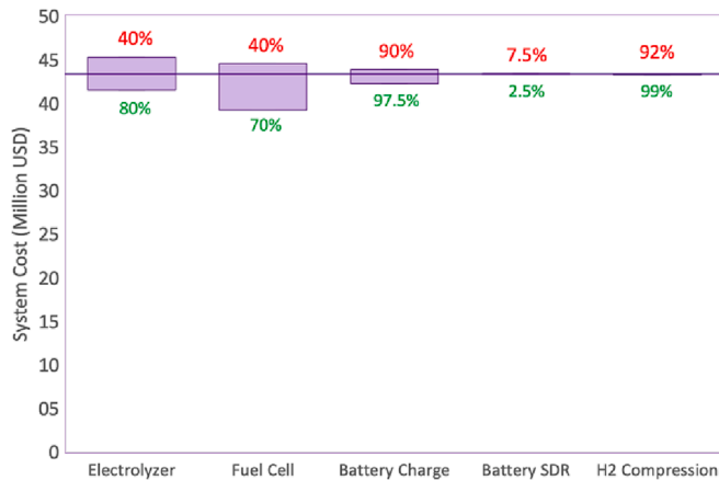
Fig. 8. Impact of Component Efficiency/Self-Discharge Rate (SDR) on Total System Cost. Efficiency ranges for each technology reflect the lowest current estimates and targeted future efficiencies. The solid line is the baseline system cost from the 2020 Hybrid Base Case. Note that little attention in the literature is given to battery self-discharge rate. Here, we scale a standard assumption of 5% monthly SDR by \pm 50\% , giving a range of 2.5%-7.5%.
