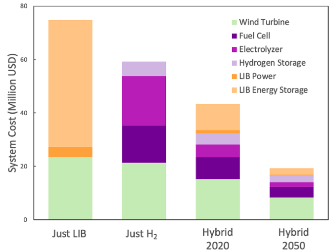
Fig. 5. Annualized Cost Breakdown for Core Cases. ‘Just LIB’ refers to a microgrid that uses only LIB for energy storage (i.e., just LIB power and LIB energy storage components) with 2020 cost and efficiency parameters; ‘Just H 2 ’ refers to using only H 2 for energy storage (i.e., comprised of electrolyzers and fuel cells for power conversion and tanks for storage); ‘2020’ is the baseline hybrid system described in section 4.1; ‘2050’ is the hybrid system assuming 2050 cost and efficiency targets/projections are achieved.
