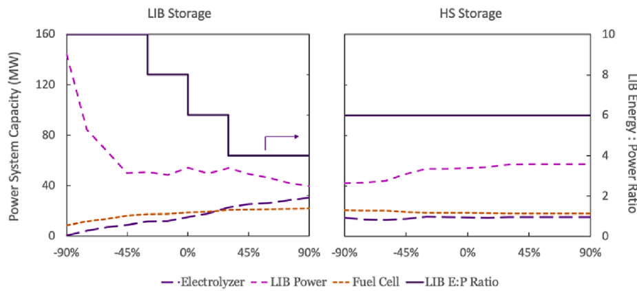
Fig. 10. Impact of Energy Storage Technology Cost on Sizing and LIB Energy-Power Ratio. The x-axis displays percentage change in annualized energy storage capacity cost in $/kWh. The left and right panels show the impact of LIB and H 2 energy storage capacity costs on system composition, respectively. Dashed lines are the power conversion components, and the solid line is the LIB energy-power ratio.
