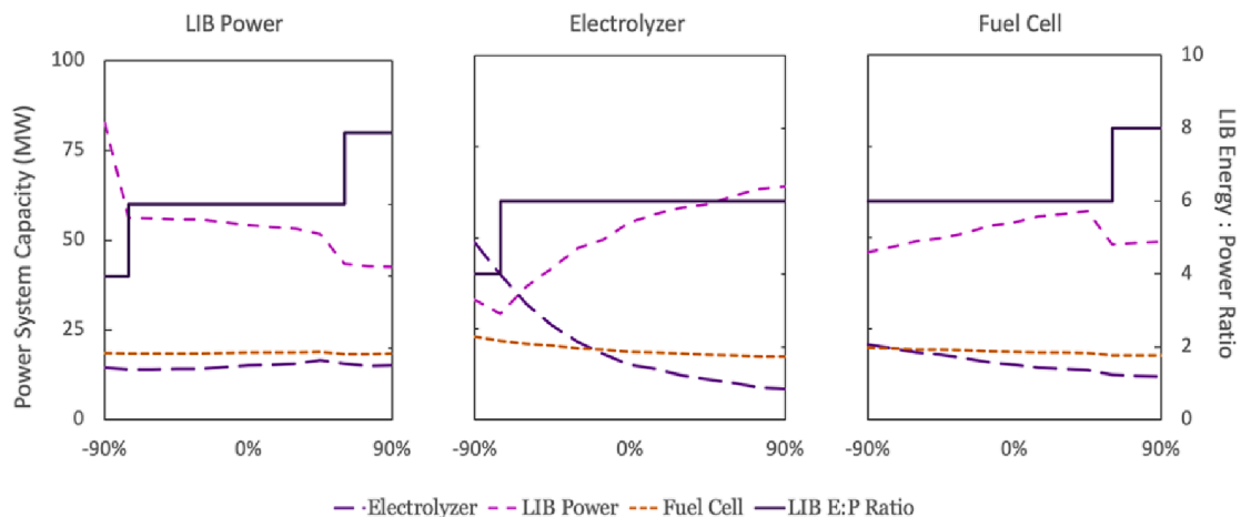
Fig. 11. Impact of Power Conversion Technology Cost on Sizing and LIB Energy-Power Ratio. The x-axis displays percentage change in annualized power conversion cost in $/kW. The left, middle, and right panels show the impact of LIB power conversion (i.e., charge and discharge), electrolyzer, and fuel cell cost on system composition, respectively. Dashed lines are the power conversion components, and the solid line is the LIB energy-power ratio.
