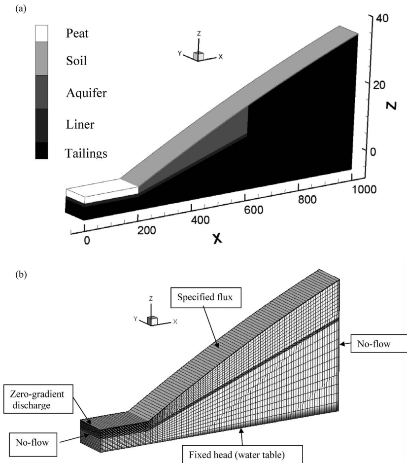
Figure 2. (a) Materials distribution and (b) finite-element grid and flow boundary conditions.
