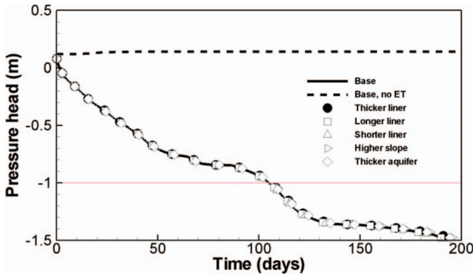
Figure 6. Steady-state case 2. Pressure response in fen because of changes in design features and using Liner II, Aquifer I properties.
