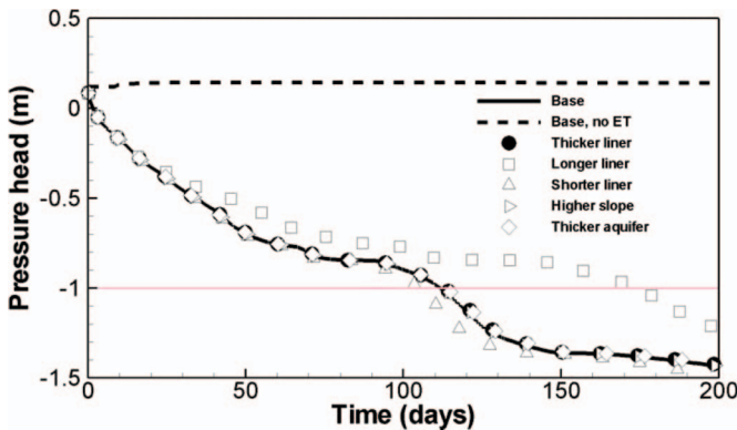
Figure 7. Steady-state case 4. Pressure response in fen due to changes in design features and using Liner II, Aquifer II properties.
