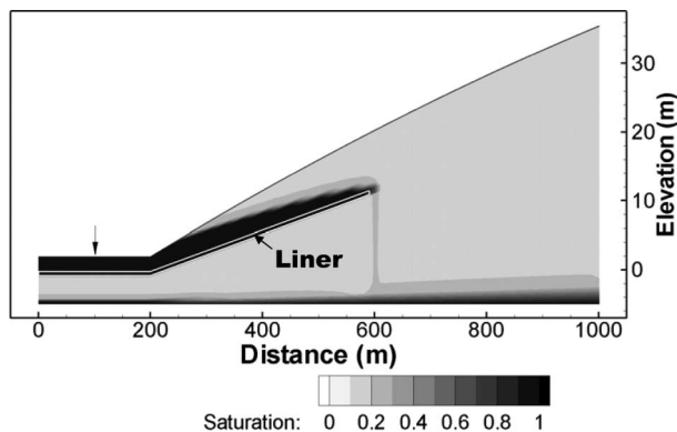
Figure 4. Initial water saturation for Liner I, Aquifer I properties with extent of liner indicated by white line. The arrow represents the position in the fen (10 cm below the surface), for which pressure is reported in the following simulations.
