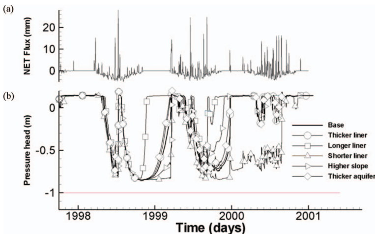
Figure 8. Transient case 1. (a) NET Flux (mm) and (b) Transient pressure response to daily climate inputs (rain, snowmelt, evaporation and transpiration) and using Liner II, Aquifer II properties.
