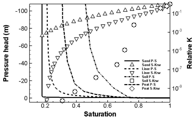
Figure 3. Moisture retention curves, where P-S denotes the pressure vs. saturation relationship and S-Krw denotes the saturation vs. relative K relationship.
