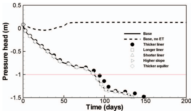
Figure 5. Steady-state case 1. Pressure response in fen because of changes in design features and using Liner I, Aquifer I properties. The horizontal grey line in this and subsequent pressure vs. time graphs represents the threshold pressure defined by Price [15].
